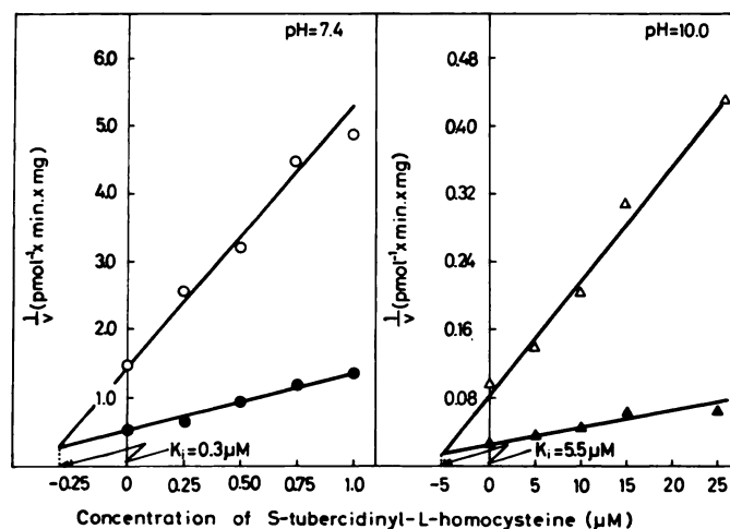
FIG. 3. Inhibition of phospholipid methyltransferase activity by S -tubercidinyl-L-homocysteine
